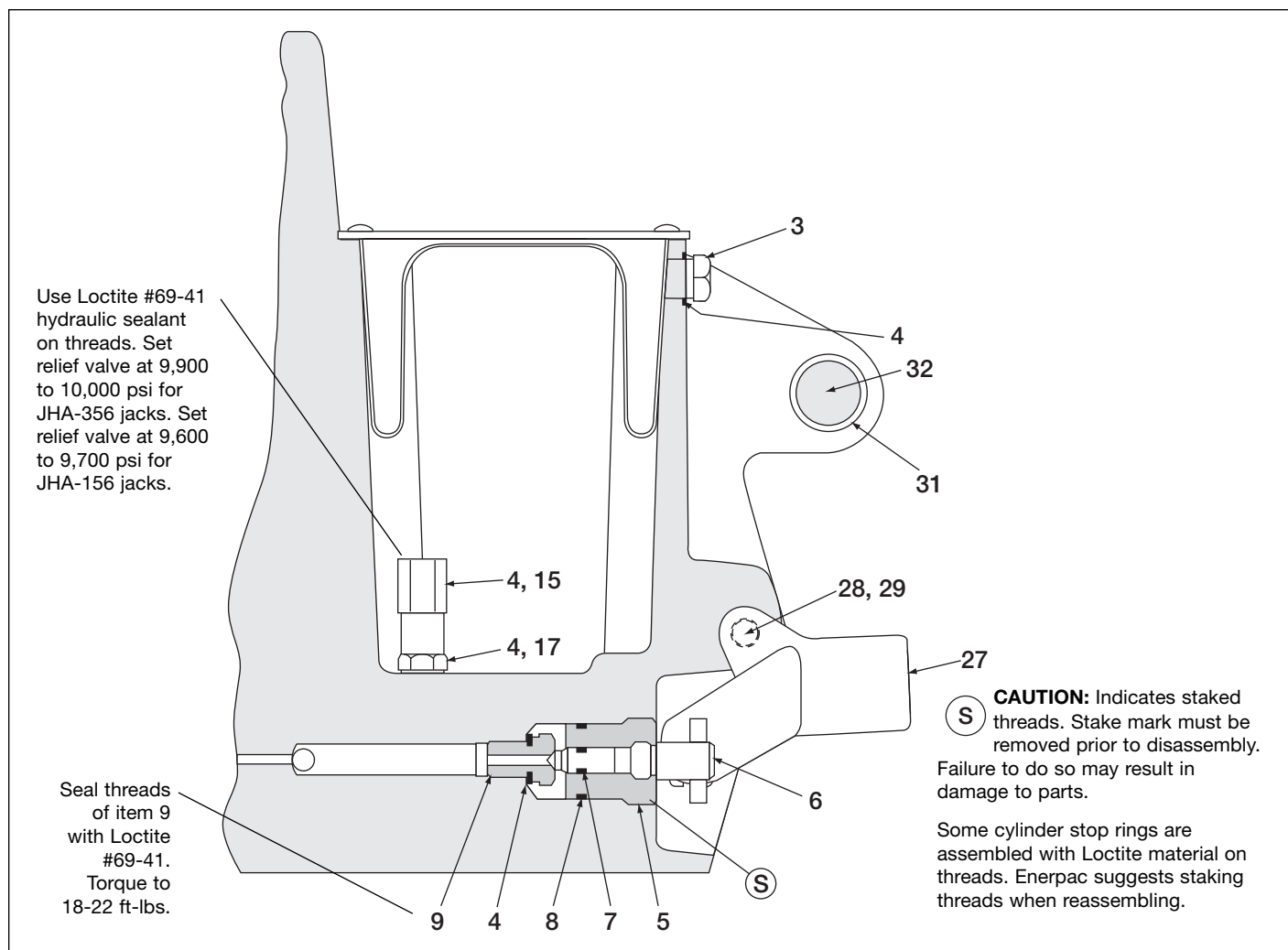
Figure 2, Section View B-B
