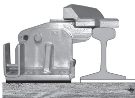
Derail shimmed
