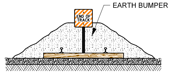
APPROACH VIEW
