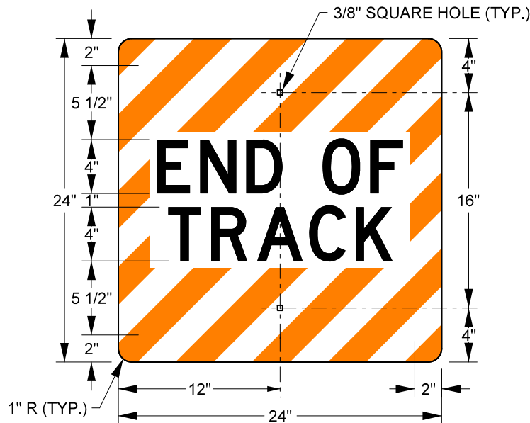
END OF TRACK SIGN ITEM NO. 393-1546
