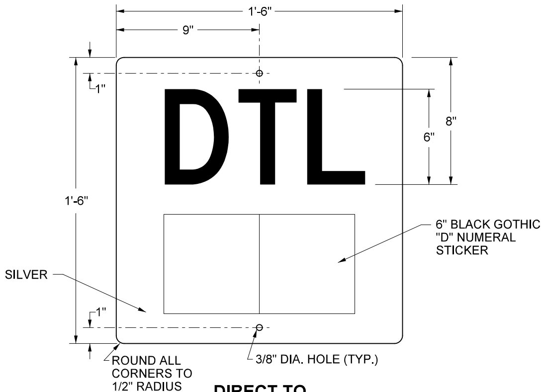
DIRECT TO LOCOMOTIVE (DTL) FUELING SIGN ITEM NO. 393-0010
