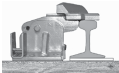
No adjustment necessary: derail base height = height of rail
